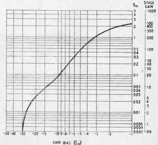
Fig. 2. Curve of Fig. 1 re-drawn with logarithmic scales for g_m and E_g .
