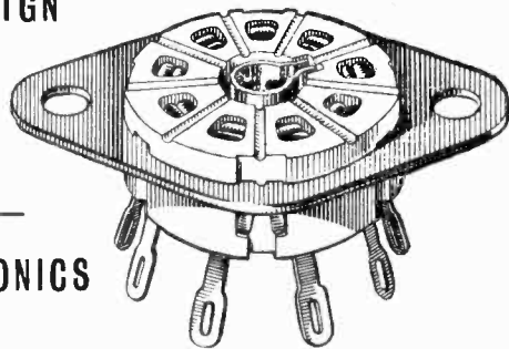
CLIX B9G valveholder for use with EF50, etc. Cat. No. VH359/9, Polystyrene Body. VH369/9, Ceramic Body.
