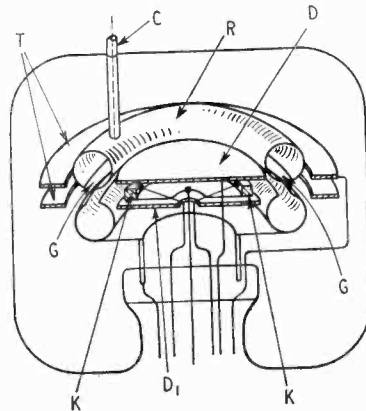
Velocity-modulated valve generator.
