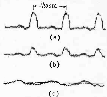
Fig. 7. Oscillograms of hum and noise with and without positive bias on heater. (a) Slider of hum-dinger earthed, (b) slider of hum-dinger at +1.5V to earth, (c) slider of hum-dinger at +4.5V to earth
