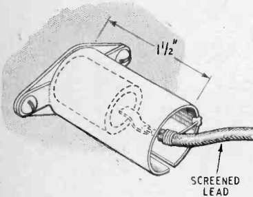
Fig. 2. Home-made sheet-metal screen for input terminal.
