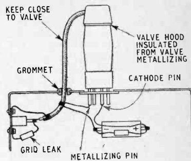
Fig. 5. A good practical layout—often quite adequate.
