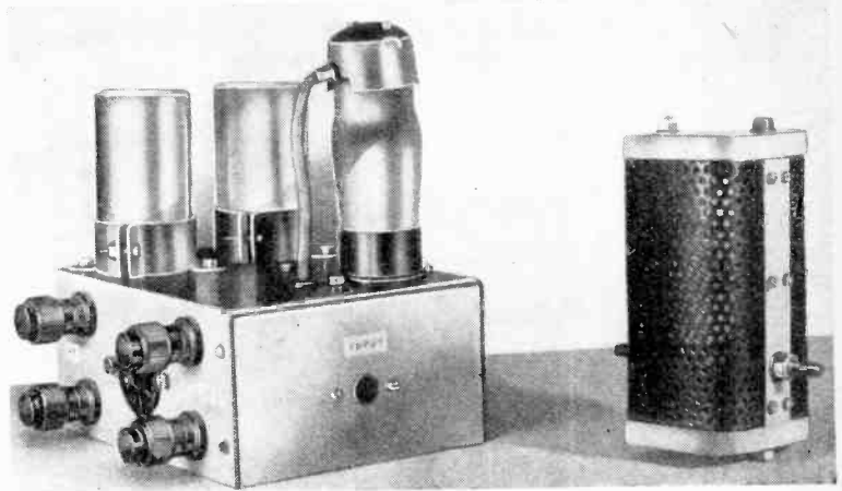
Typical microphone pre-amplifier and (right) experimental ribbon microphone.
